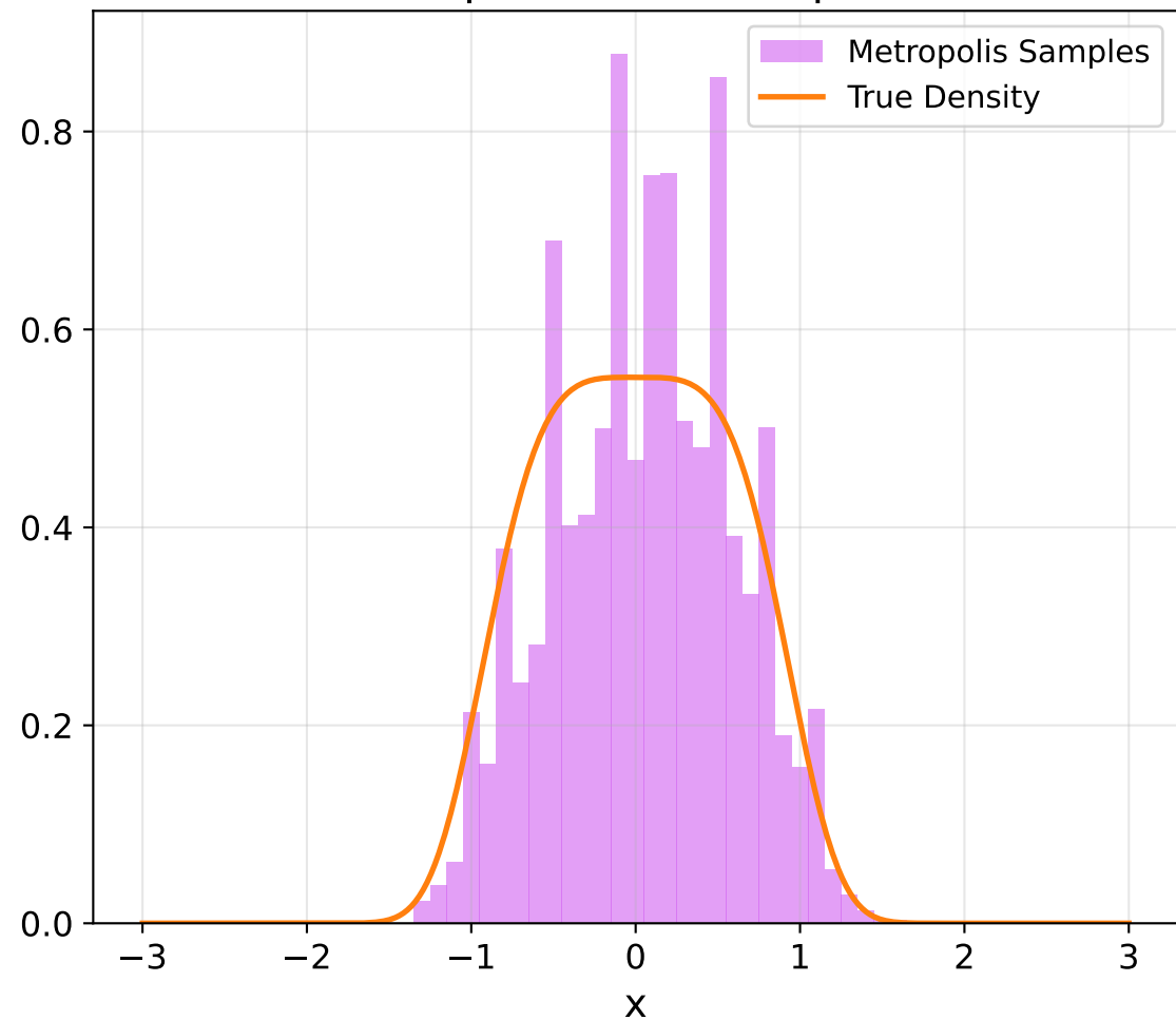
Random Walk (Step=0.075), Acceptance Rate=0.96
